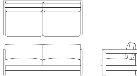
3Pソファ L08710S [W/1820 D/830 H/760 SH/400] OIL WN
